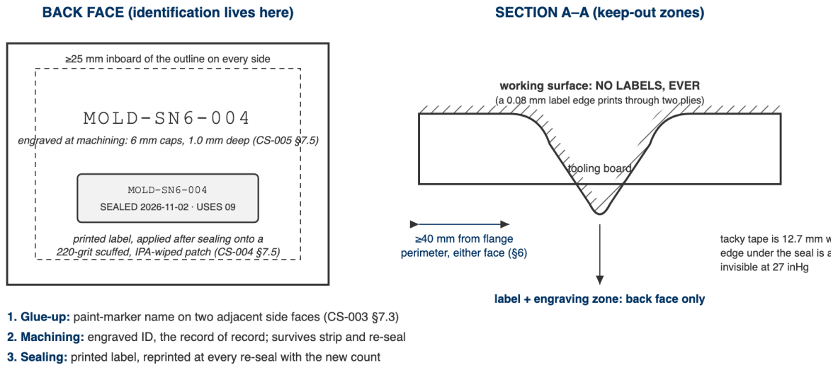
Figure 2: Where a mold’s identity lives, and the two keep-out zones: never the working surface, never within 40 mm of the flange perimeter on either face.
